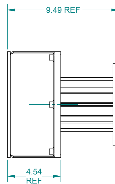
DETAIL OF ASSEMBLY SCALE:1:4
