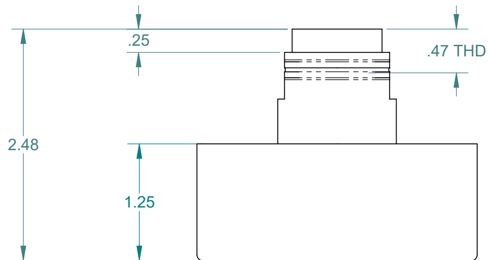
DETAIL OF TPLP30 SCALE:1:1
